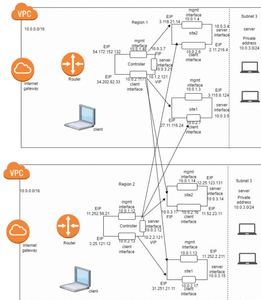
Figure 68 : 3NIC-6VM-2RG-GSLB Deployment Topology
