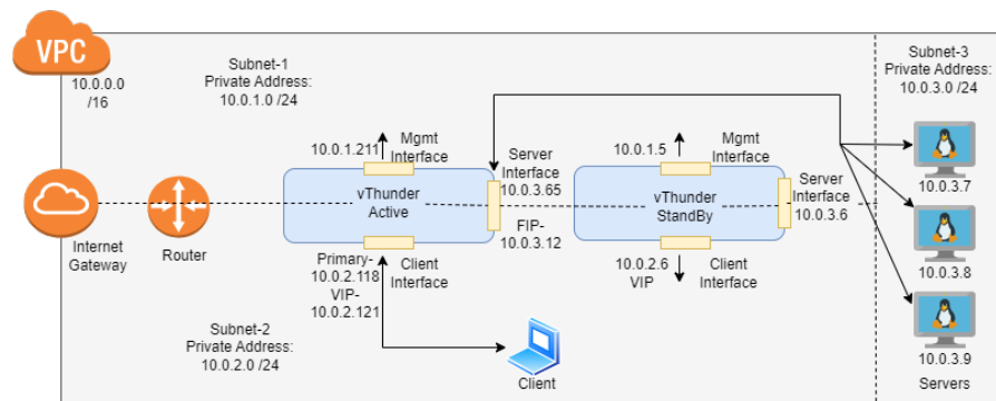
Figure 34 : 3NIC-2VM-HA-GLM-PVTVIP Deployment Topology
