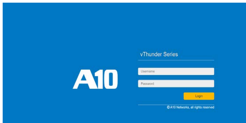
Figure 39 : vThunder GUI
