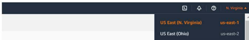
Figure 74 : Region dropdown
