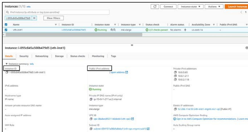
Figure 40 : vThunder instance
