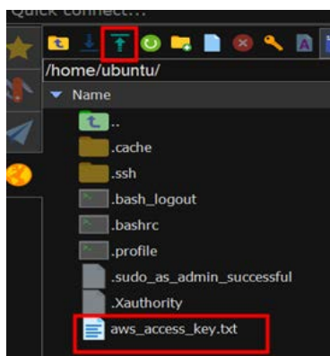
Figure 28 : MobaXterm Upload
