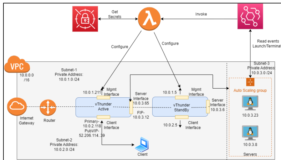
Figure 49 : 3NIC-2VM-HA-GLM-PUBVIP-BACKAUTO Deployment Topology
