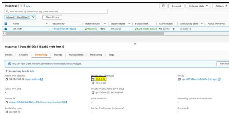
Figure 10 : vThunder instance
