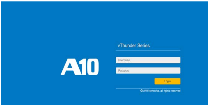
Figure 78 : vThunder GUI
