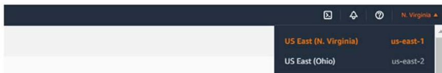
Figure 70 : Region dropdown
