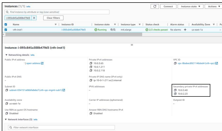
Figure 33 : vThunder instance 1
