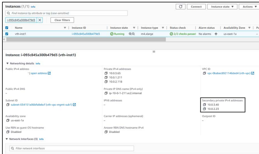
Figure 48 : vThunder instance 1
