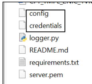
Figure 2 : CFT folder
