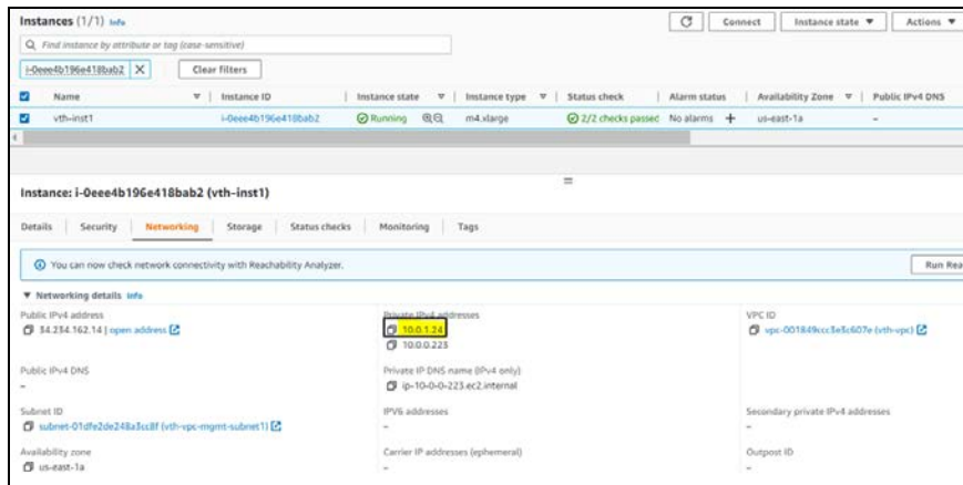
Figure 19 : vThunder instance
