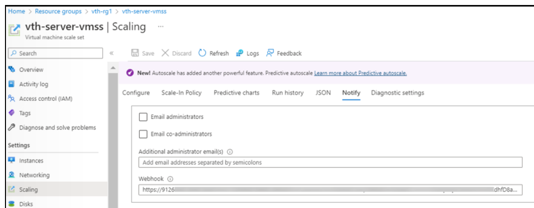
Figure 153 : VMSS-Scaling - Notify tab
