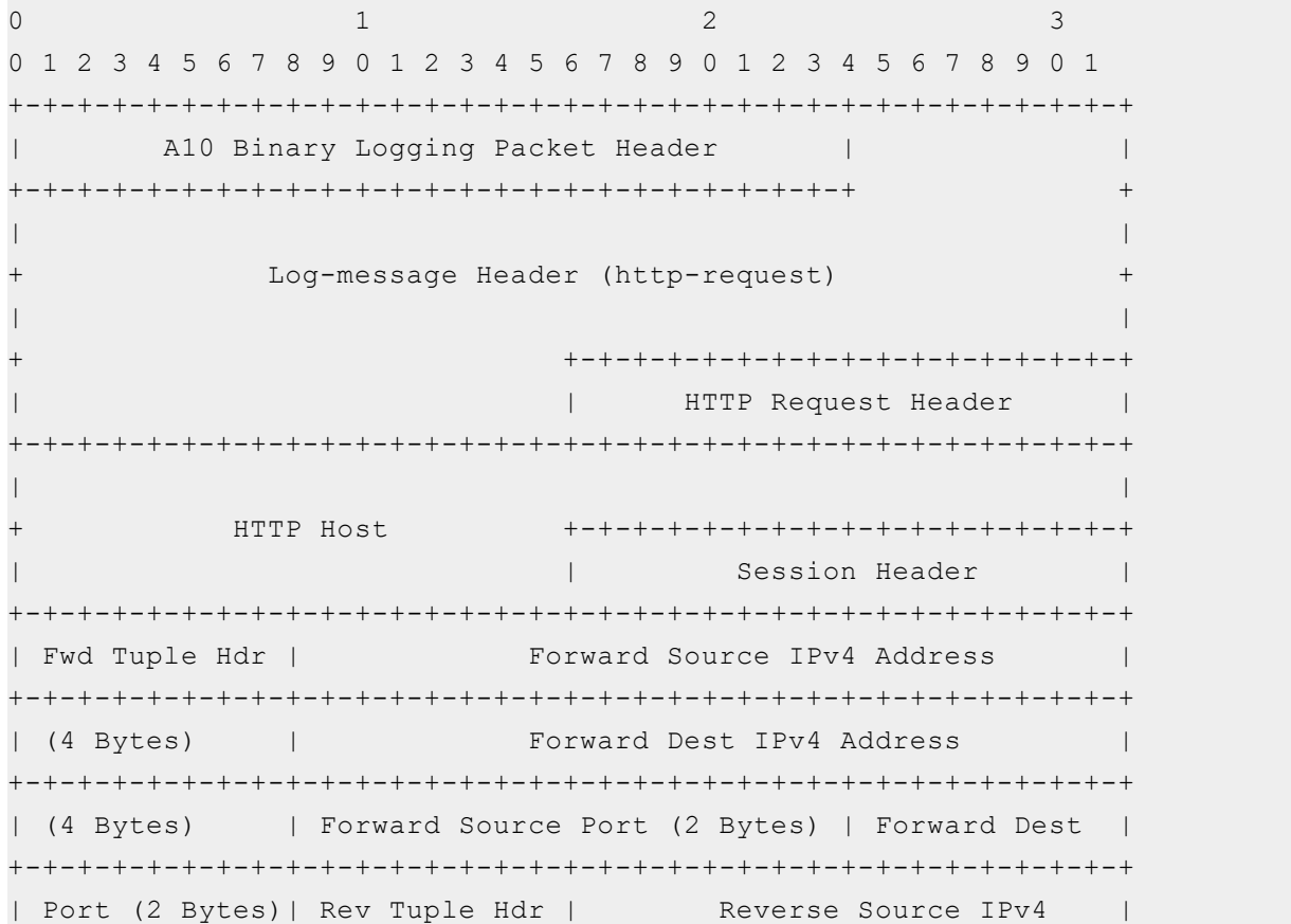
Figure 59 : Binary Logging Format - include client mobile number (MSISDN), HTTP request information including hostname, HTTP method, and Layer 4 session information
