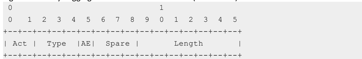
Figure 9 : Binary Logging Format - Fixed-NAT header (ACOS 2.8.2)
