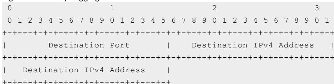
Figure 28 : Binary Logging Format - destination-info extension: LSN
