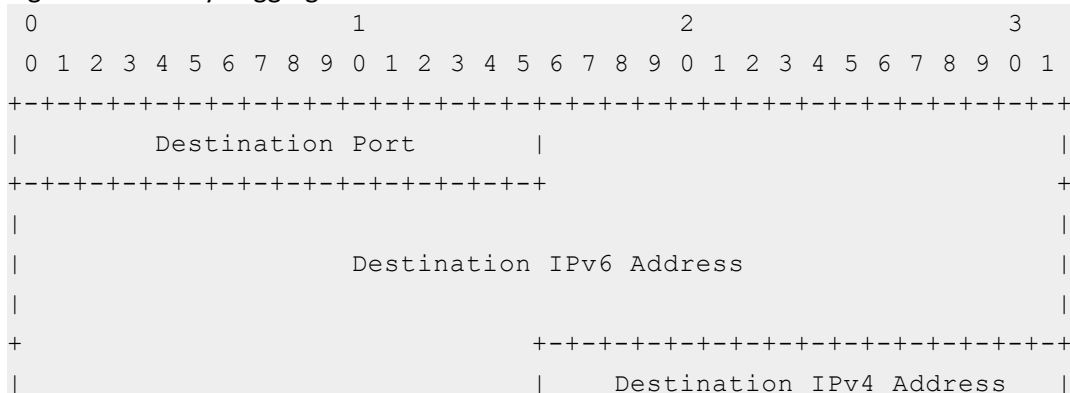
Figure 30 : Binary Logging Format - destination-info extension: DS-Lite
