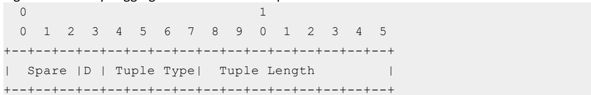
Figure 18 : Binary Logging Format - forward tuple header
