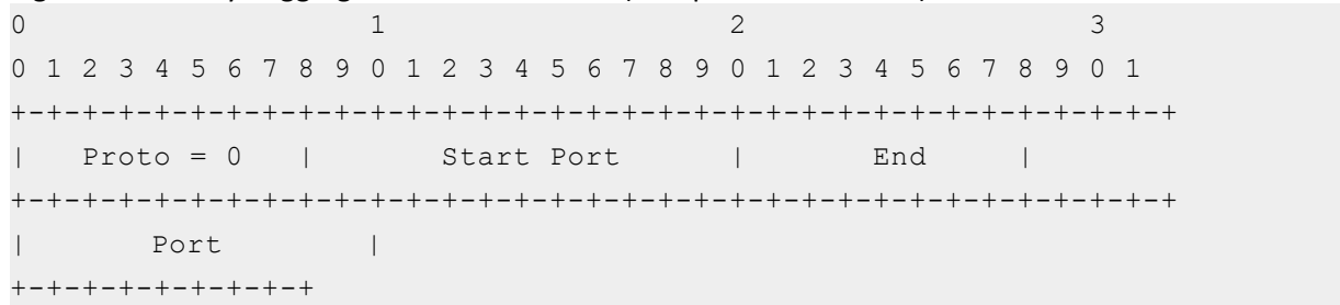
Figure 51 : Binary Logging Format - Fixed-NAT (NAT port information)
