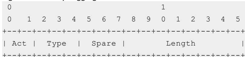
Figure 37 : Binary Logging Format - Fixed-NAT header
