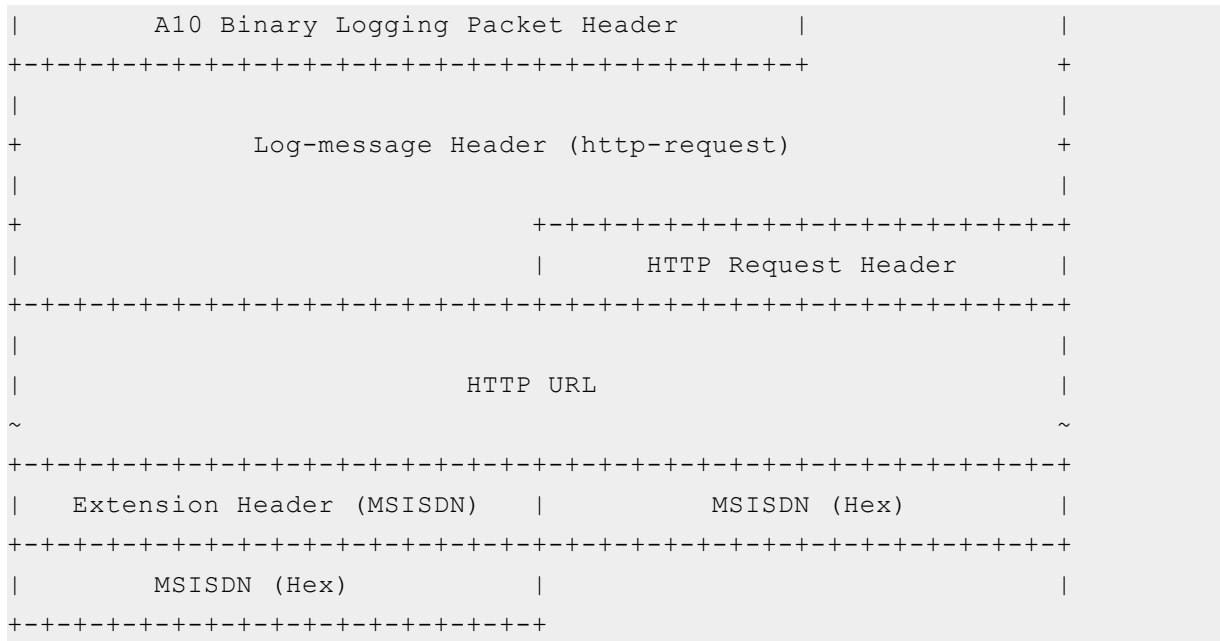
Figure 59 : Binary Logging Format - include client mobile number (MSISDN), HTTP request information including hostname, HTTP method, and Layer 4 session information
