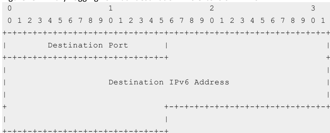
Figure 30 : Binary Logging Format - destination-info extension: DS-Lite
