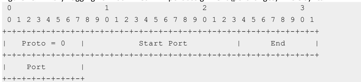
Figure 41 : Binary Logging Format - Fixed-NAT port assignment (port ranges) - 2.6.2 syntax
