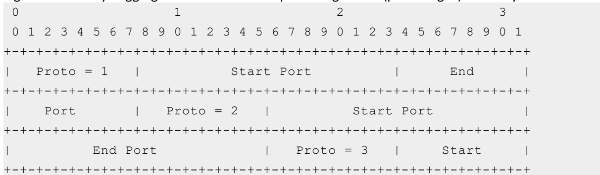
Figure 41 : Binary Logging Format - Fixed-NAT port assignment (port ranges) - 2.6.2 syntax
