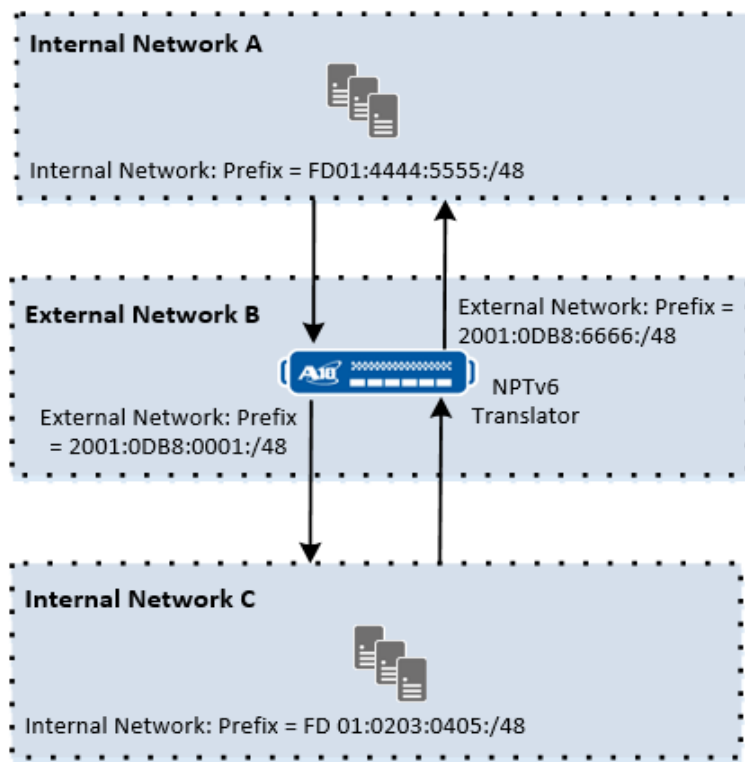
Figure 37 : Prefix Translation Between Two Private Networks
