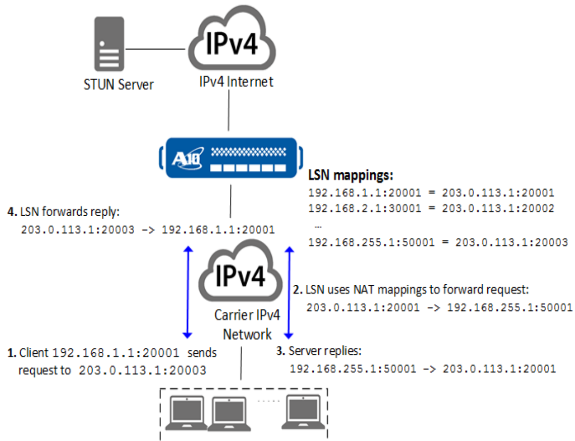
Figure 4 : LSN NAT – Hairpinning
