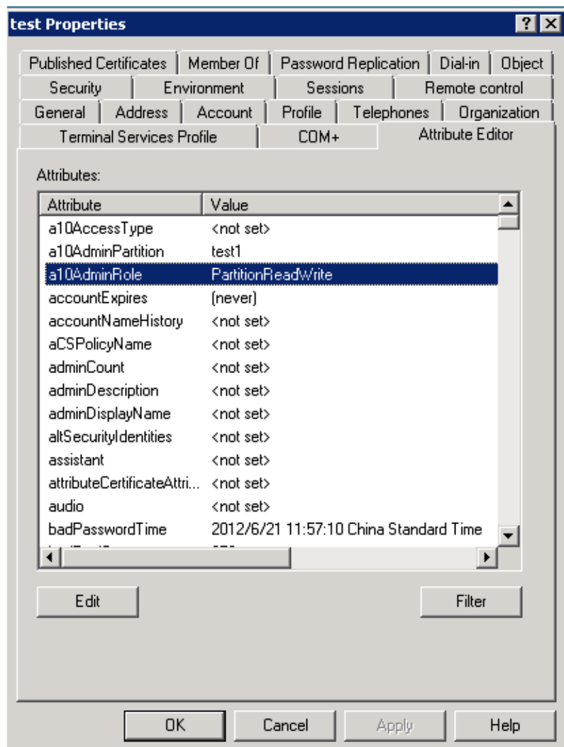
Figure 14 : LDAP Server Configuration
