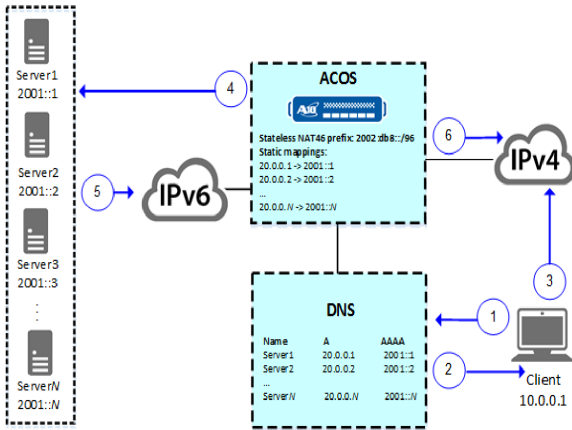
Figure 34 : Stateless NAT46
