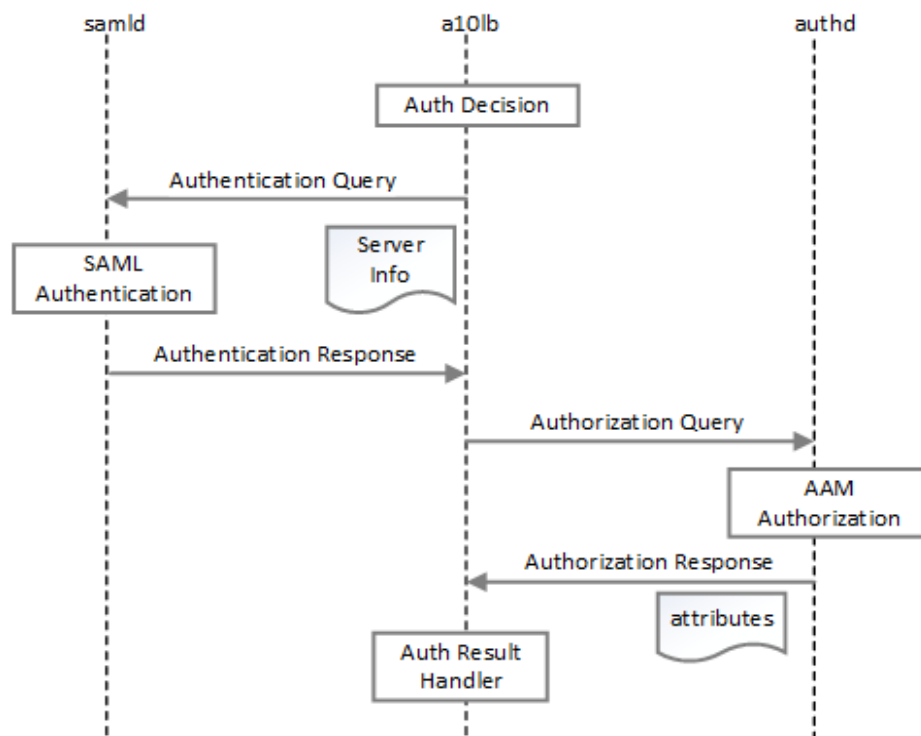
Figure 20 : Workflow for SAML and RADIUS Authentication and Authorization
