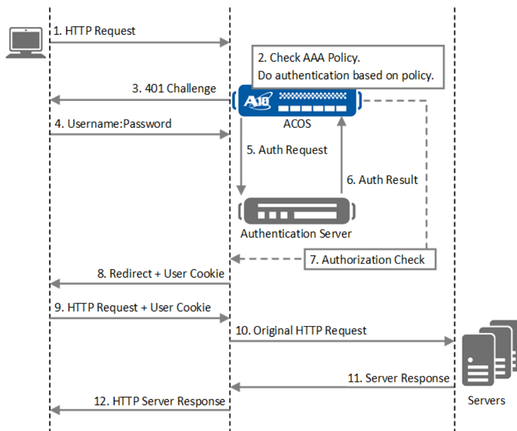
Figure 2 : Authorization Policy Workflow
