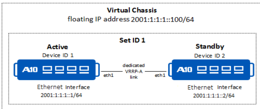
Figure 13 : Sample First-Time aVCS Deployment Topology - IPv6
