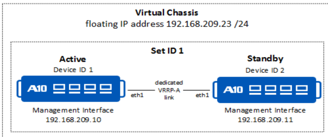
Figure 12 : Sample First-Time aVCS Deployment Topology - IPv4
