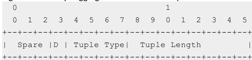
Figure 18 : Binary Logging Format - forward tuple header
