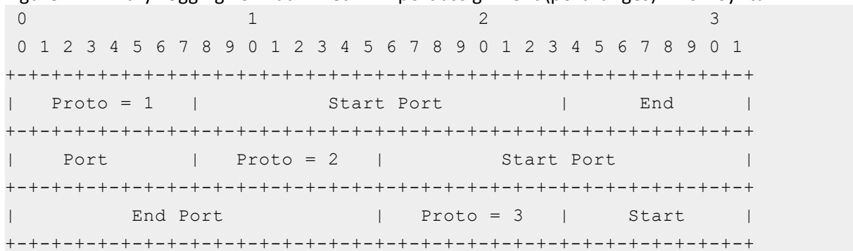
Figure 41 : Binary Logging Format - Fixed-NAT port assignment (port ranges) - 2.6.2 syntax
