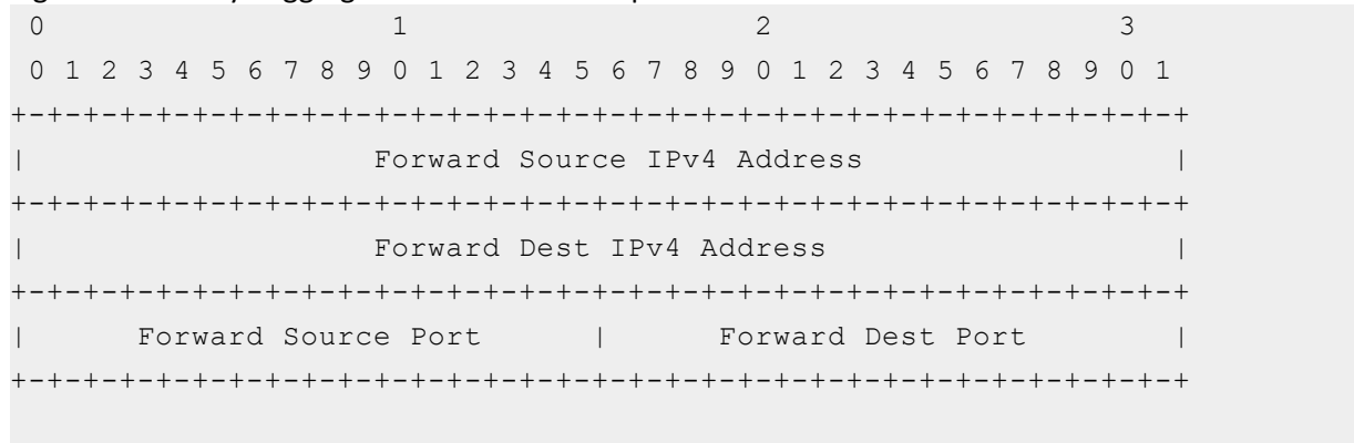
Figure 20 : Binary Logging Format - forward tuple: IPv6
