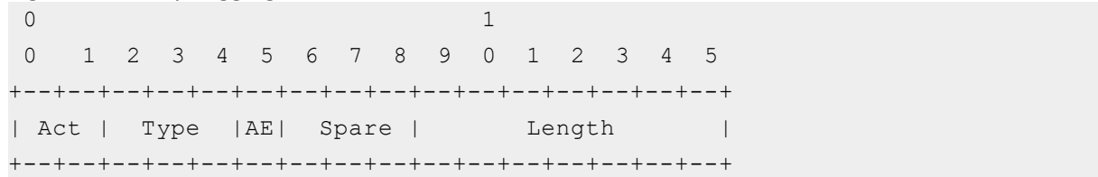
Figure 9 : Binary Logging Format - Fixed-NAT header
