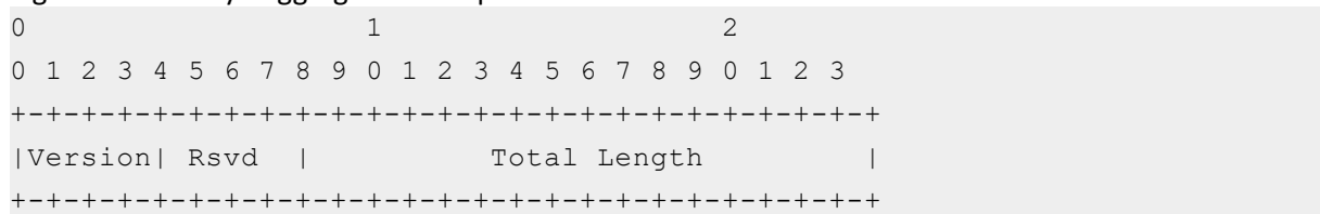
Figure 15 : Binary Logging Format - packet header
